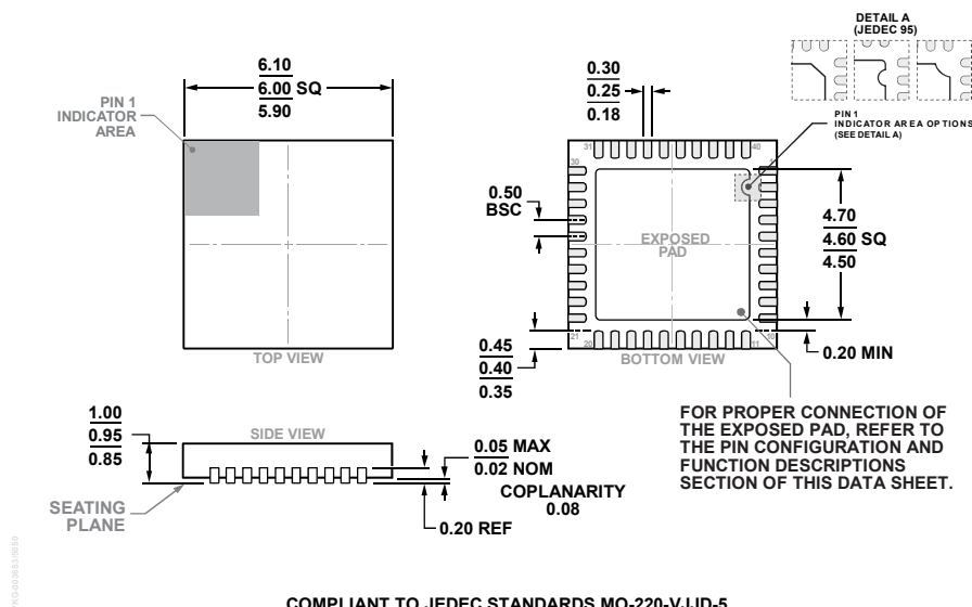
Figure 59. 40-Lead Lead Frame Chip Scale Package [LFCSP] 6 mm × 6 mm Body and 0.95 mm Package Height (CP-40-15)
