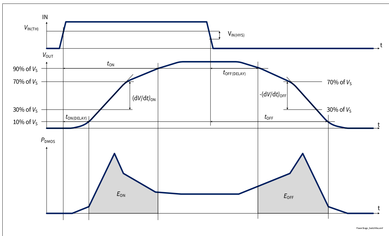
Figure 15 Switching a Resistive Load
