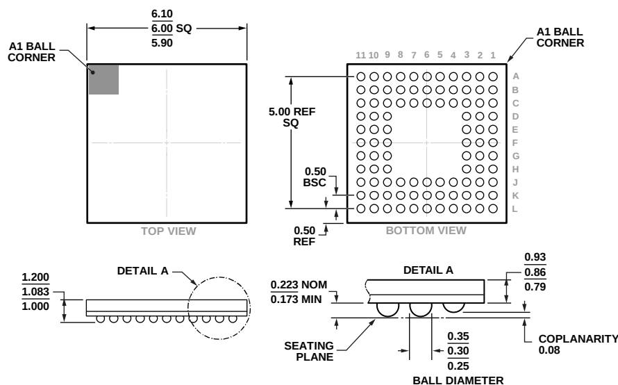
COMPLIANT TO JEDEC STANDARDS MO-195-AC WITH THE EXCEPTION TO BALL COUNT. Figure 16. 96-Ball Chip Scale Package Ball Grid Array [CSP_BGA] (BC-96-2) Dimensions shown in millimeters
