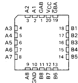
SN54ALS', SN54AS' ... FK PACKAGE (TOP VIEW)
