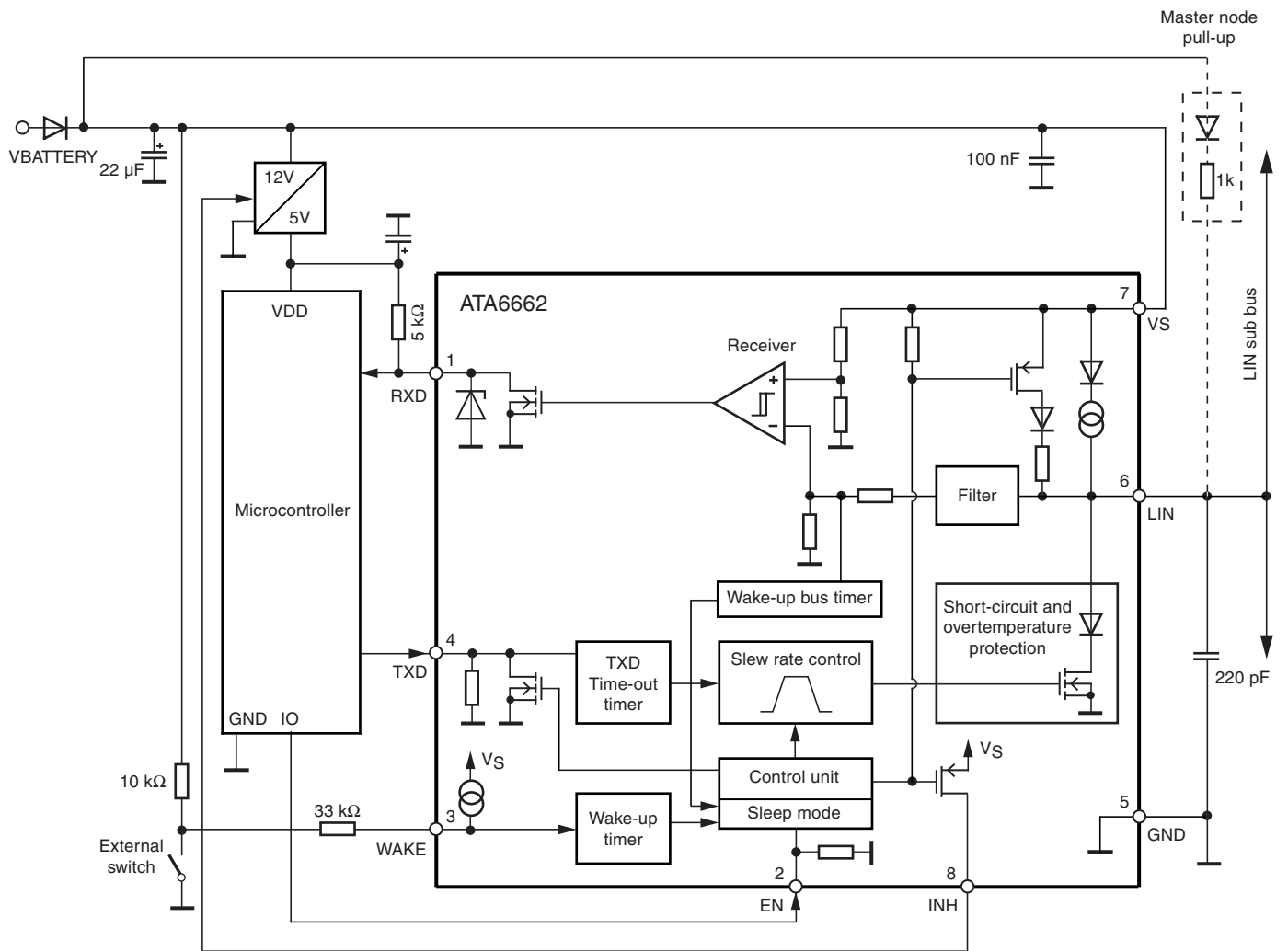
Figure 6-2. Application Circuit
