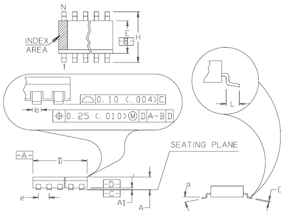
20 LEAD TSSOP
