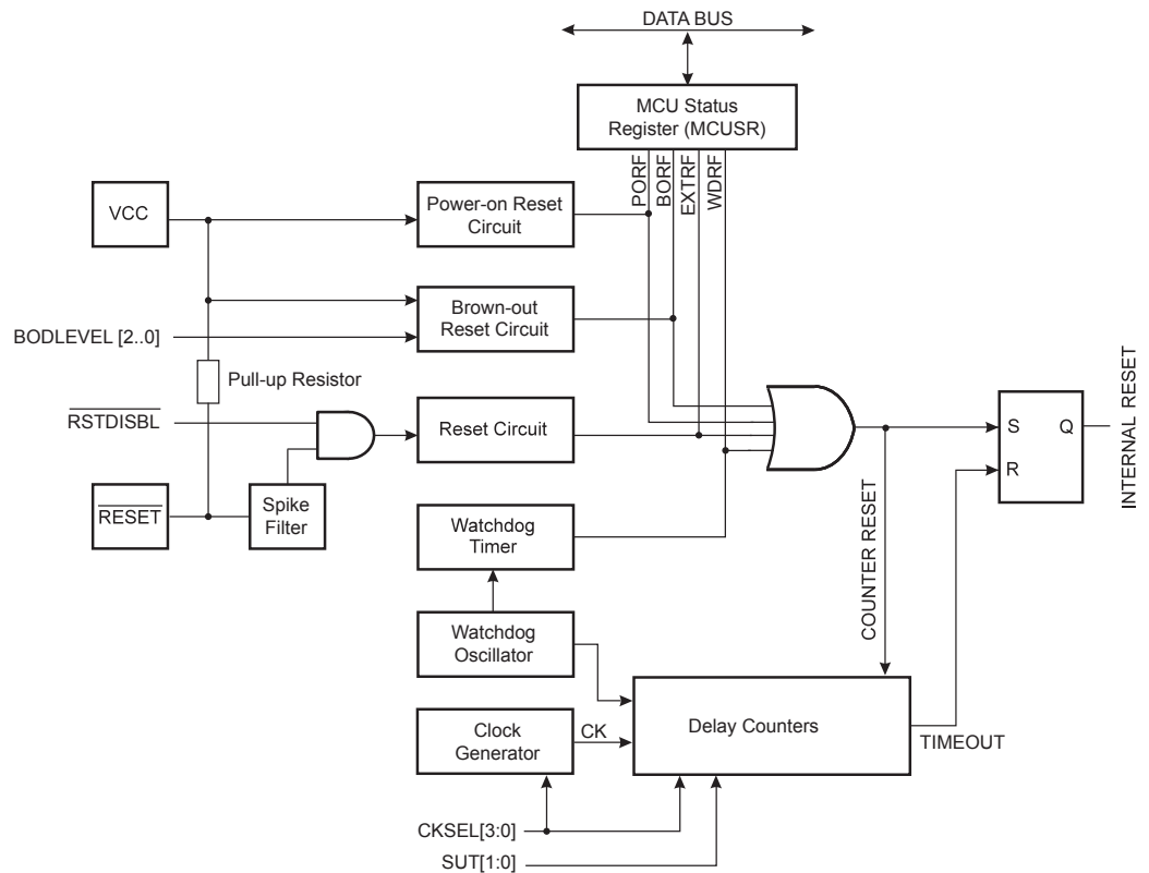
Figure 6-1. Reset Circuit
