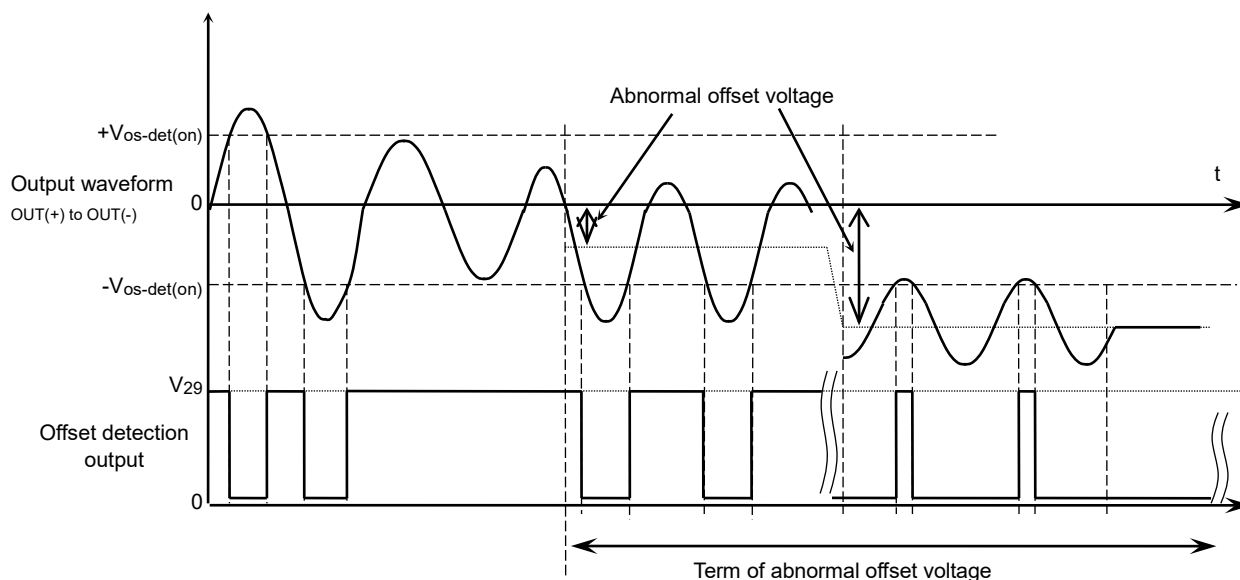
Figure 7.8 Output waveform of Pin 29
