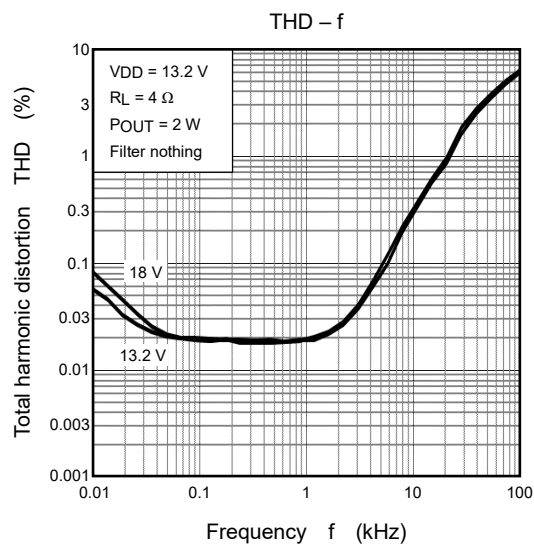
Figure 13.3 Frequency Characteristics of Total Harmonic Distortion
