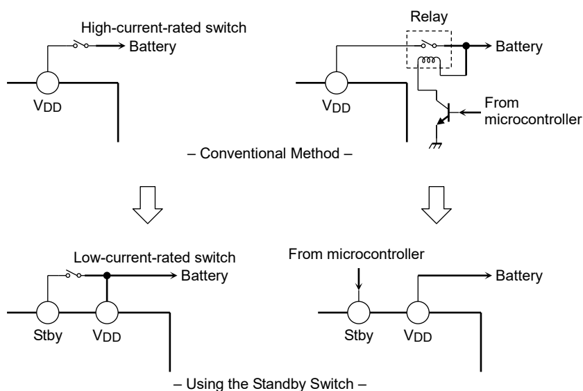
Figure 7.2 Standby switch
