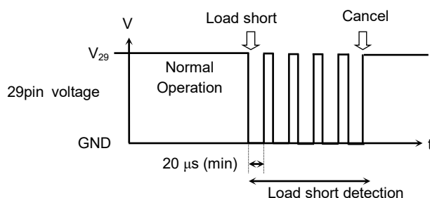
Figure 7.11 Pin 29 output waveform at load short
