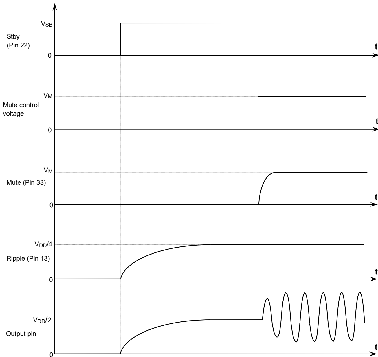
Figure 7.6 Mute off sequence after standby-off
