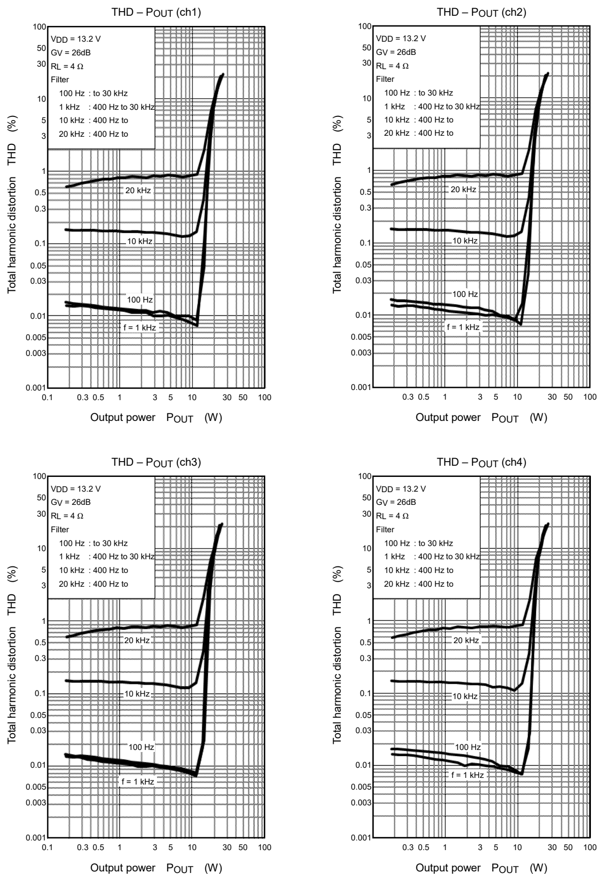
Figure 13.1 Total Harmonic Distortion of Each Frequency ( R_L = 4\ \Omega )
