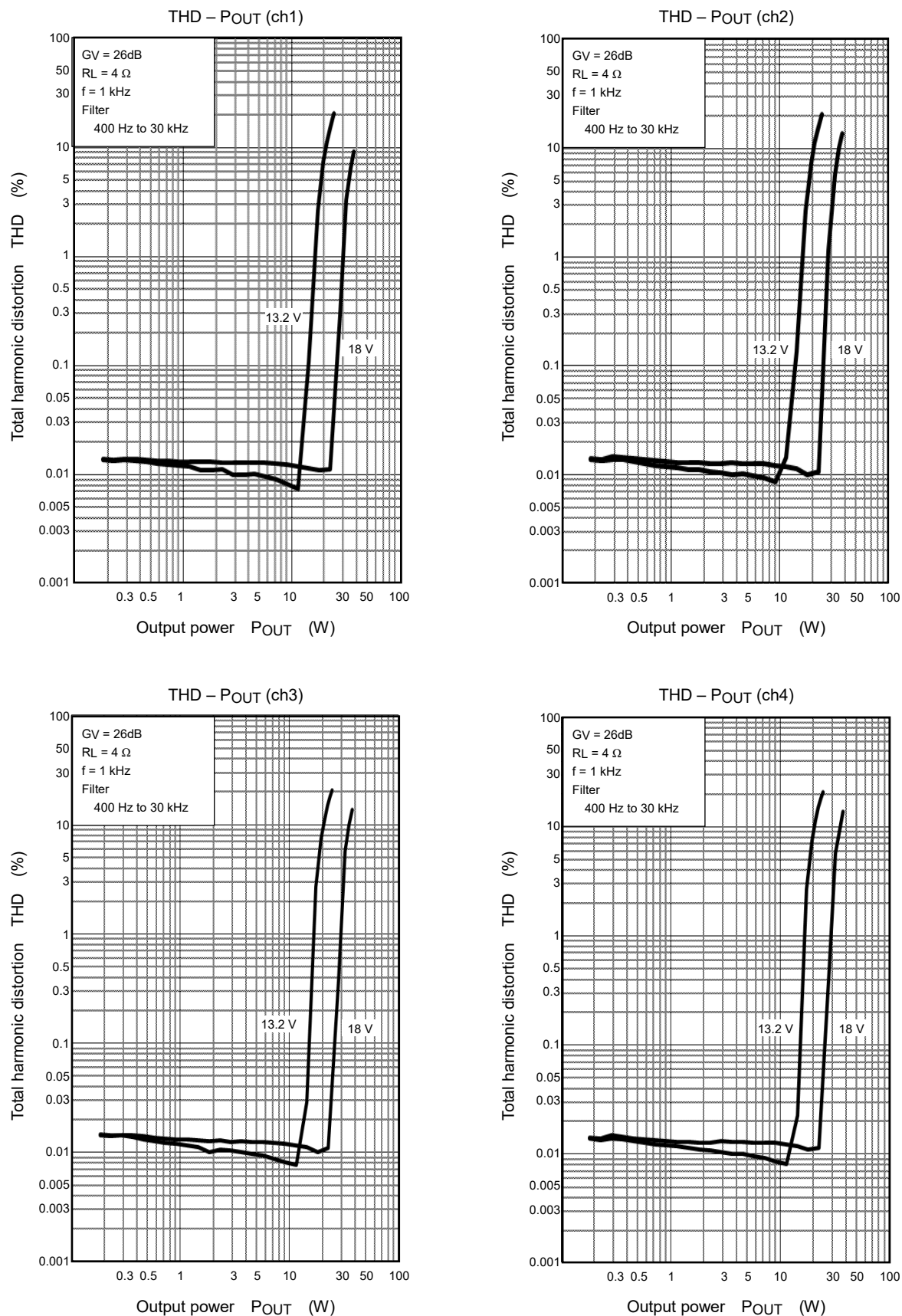
Figure 13.2 Total Harmonic Distortion by Power-supply Voltage ( R_L = 4 \Omega )
