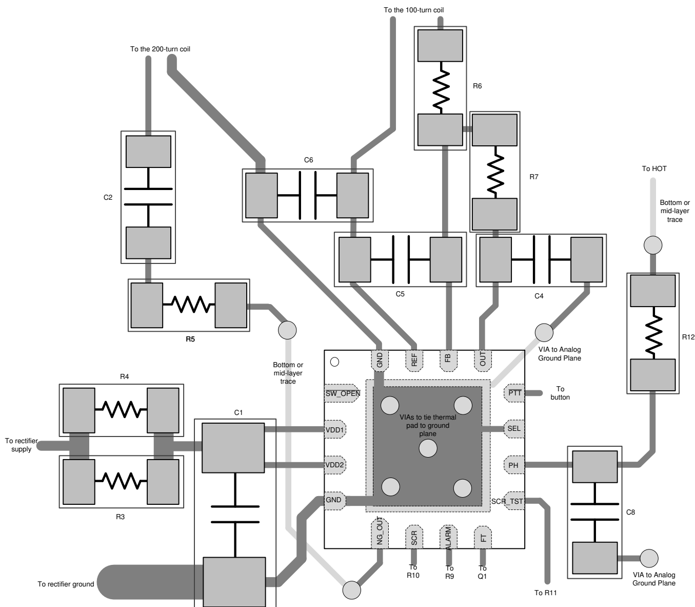
Figure 21. AFE3010 Layout Example
