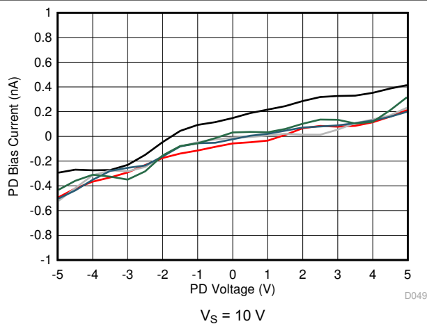
V_S = 10\text{ V} Figure 6-51. Power-Down Bias Current vs Power-Down Voltage
