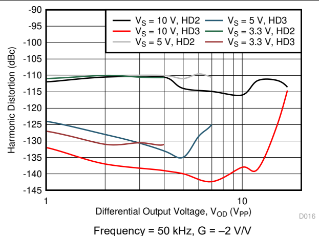
Figure 6-40. Harmonic Distortion vs Differential Output Voltage
