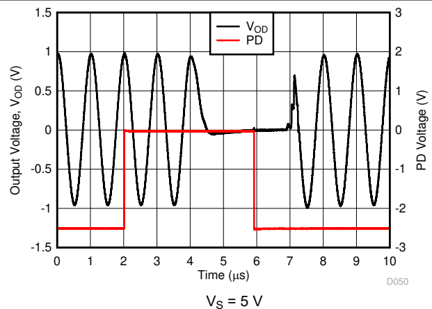
V_S = 5\text{ V} Figure 6-52. Turnon and Turnoff Timing
