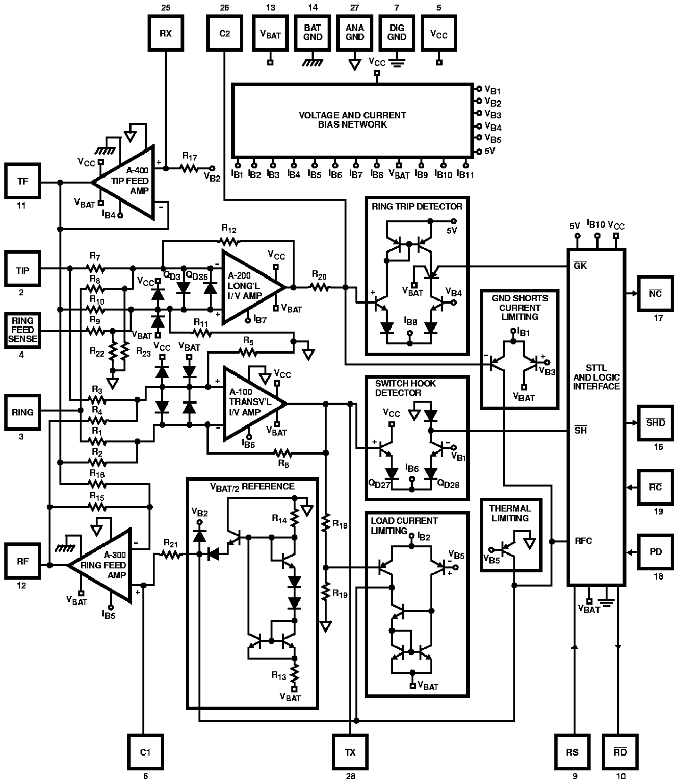
FIGURE 8. FUNCTIONAL SCHEMATIC
