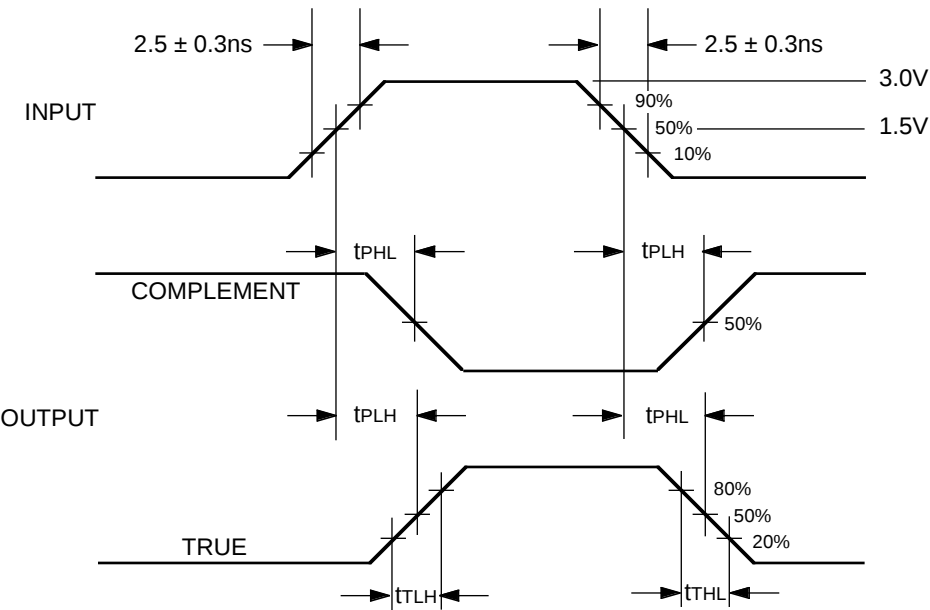
Propagation Delay and Transition Times
