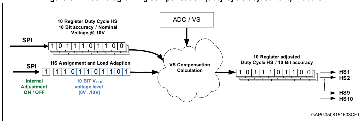
Figure 51. Block diagram V_{\text{S}} compensation (duty cycle adjustment) module
