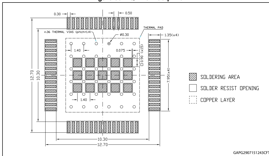
Figure 63. LQFP-64 footprint
