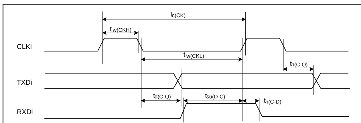
Figure 5.12 Serial Interface
