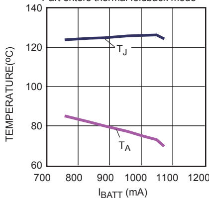
CC Charge Current vs. Temp Zoom In
