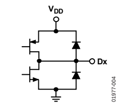
Figure 38. Digital Output Circuit
