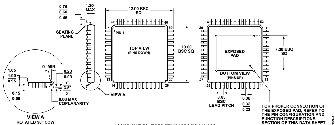
Figure 47. 52-Lead Thin Quad Flat Package, Exposed Pad [TQFP_EP] (SV-52-2)
