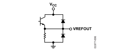
Figure 39. Voltage Reference Output Circuit
