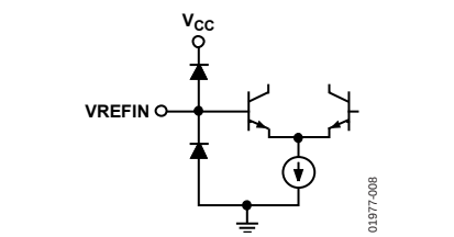
Figure 36. Voltage Reference Input Circuit
