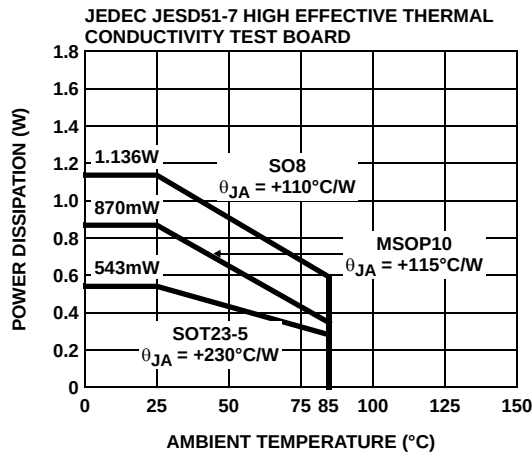
FIGURE 33. PACKAGE POWER DISSIPATION vs AMBIENT TEMPERATURE
