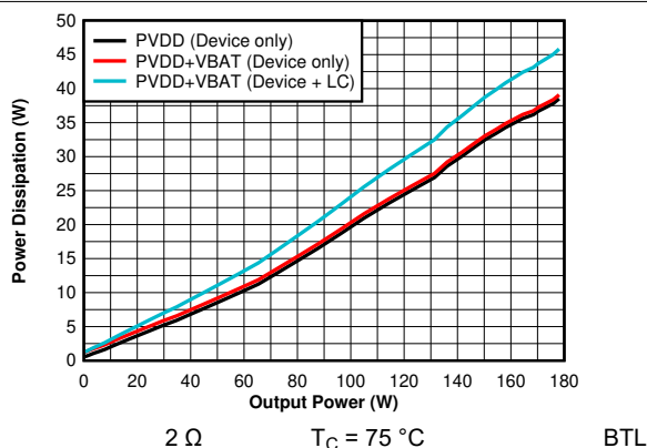
Figure 6-58. Power Dissipation vs Output Power - 2 \Omega
