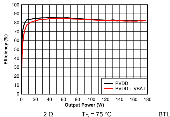
Figure 6-56. Efficiency vs Output Power - 2 \Omega
