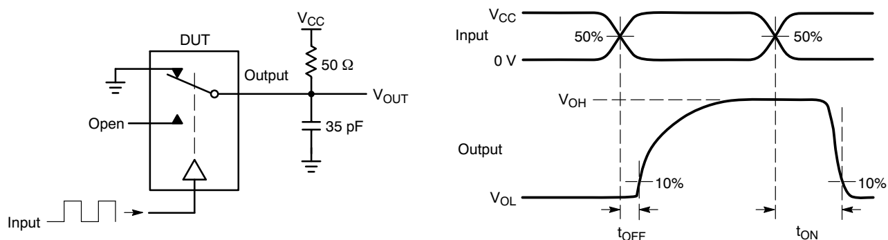
Figure 3. t_{ON} / t_{OFF} V_{is} = GND
