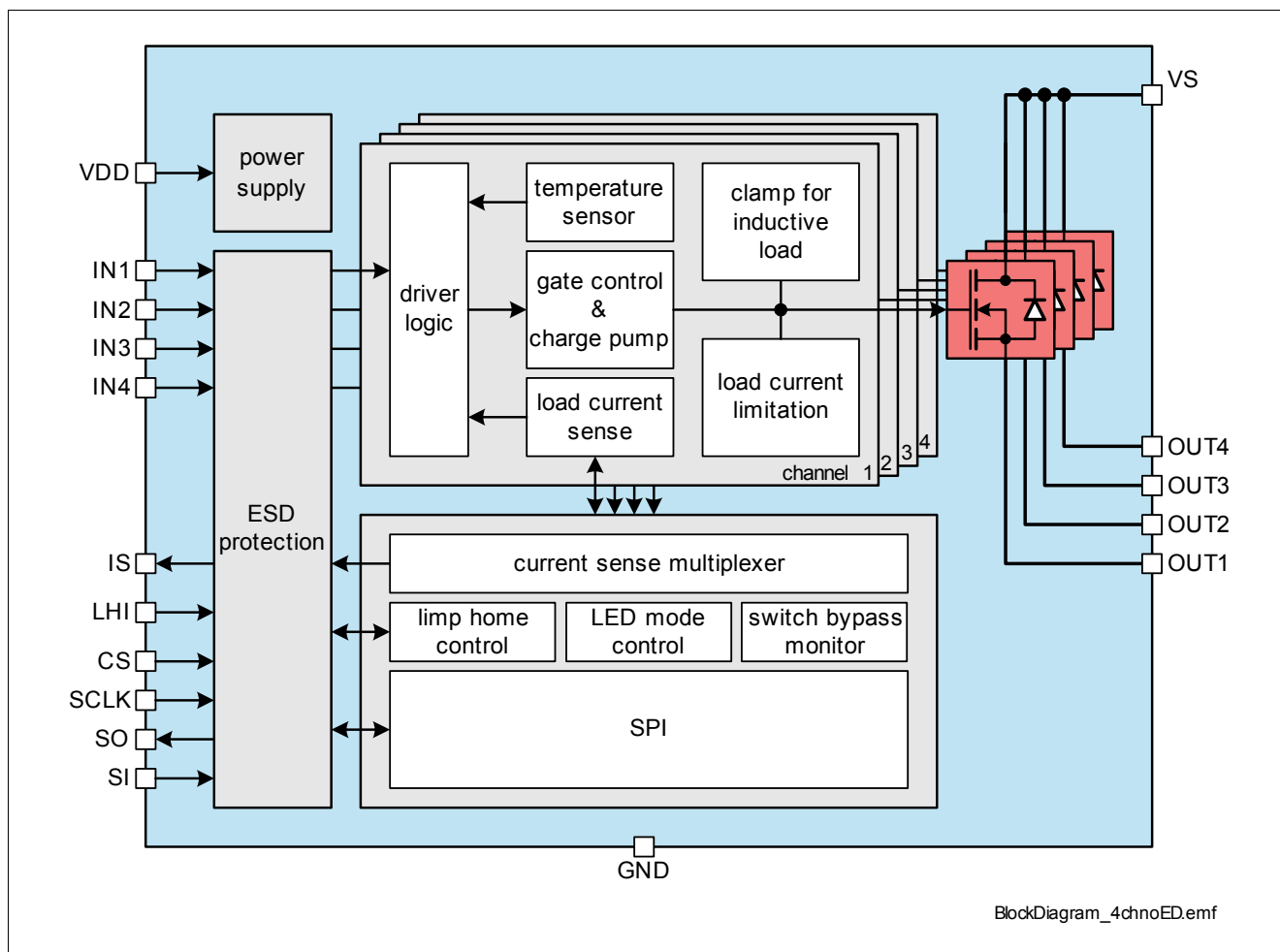
Figure 1 Block Diagram BTS54220-LBB
