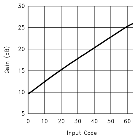
Gain vs. Input Code
