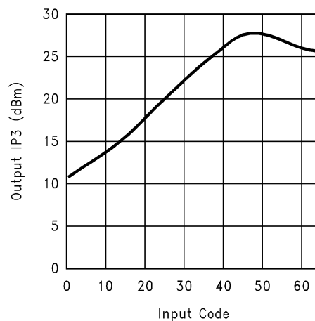
Output 3rd Order Intercept vs. Input Code
