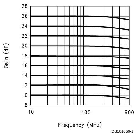
Frequency Response vs. Gain Setting
