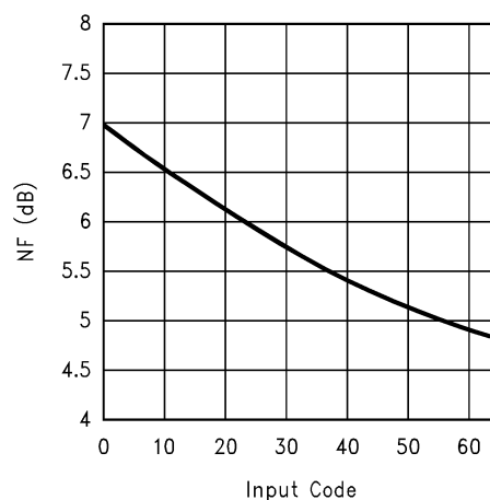
Noise Figure vs. Input Code
