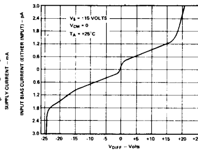
Figure 8. Input Bias Current Versus Input Differential Voltage
