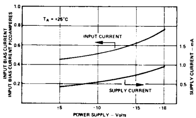
Figure 7. Input Bias Current and Supply Current Versus Supply Voltage
