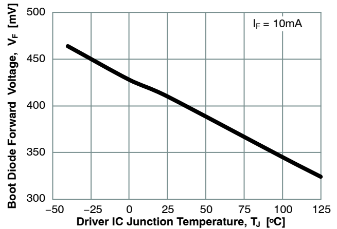
Figure 25. Boot Diode Forward Voltage vs. Temperature
