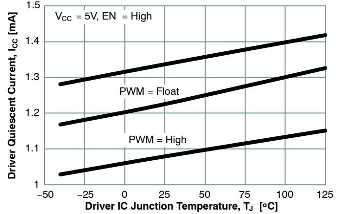
Figure 27. Driver Quiescent Current vs. Temperature
