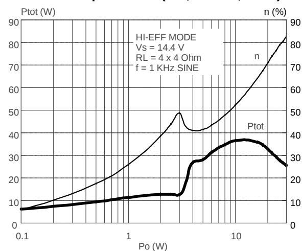
Figure 13. Power Dissipation &amp; Efficiency vs. Output Power (4W, HI-EFF, SINE)
