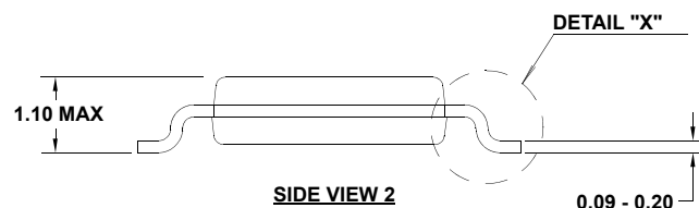
SIDE VIEW 2
