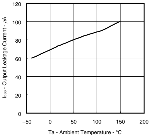
OUTPUT LEAKAGE CURRENT vs. AMBIENT TEMPERATURE
