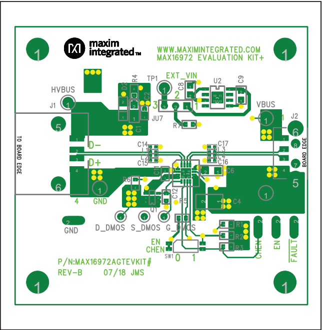
MAX16972A EV Kit PCB Layout (TQFN)—Component Side
