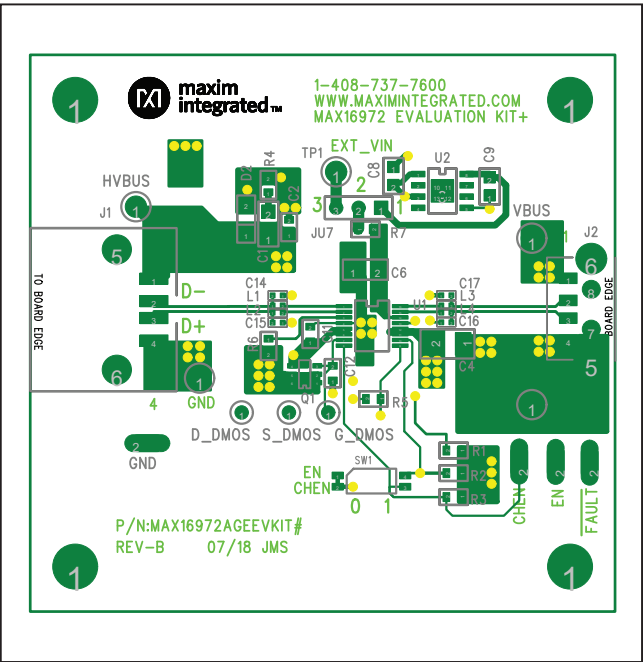
MAX16972A EV Kit PCB Layout (QSOP)—Component Side
