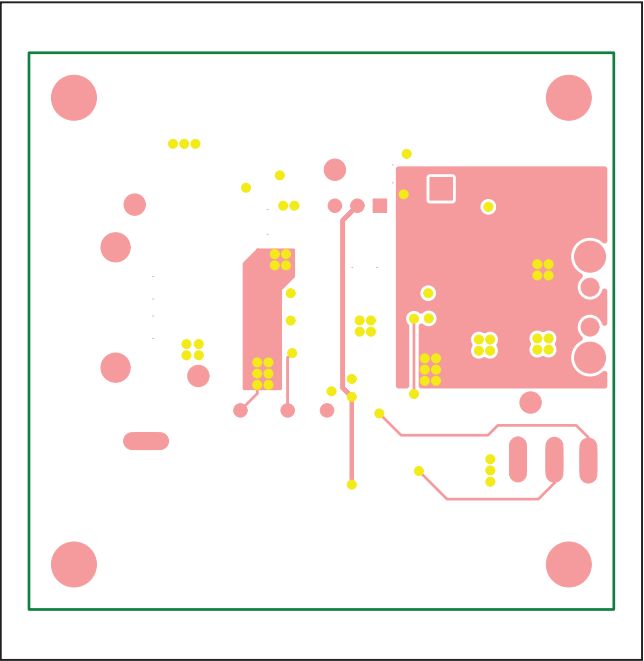
MAX16972A EV Kit PCB Layout (QSOP)—Inner Layer 3
