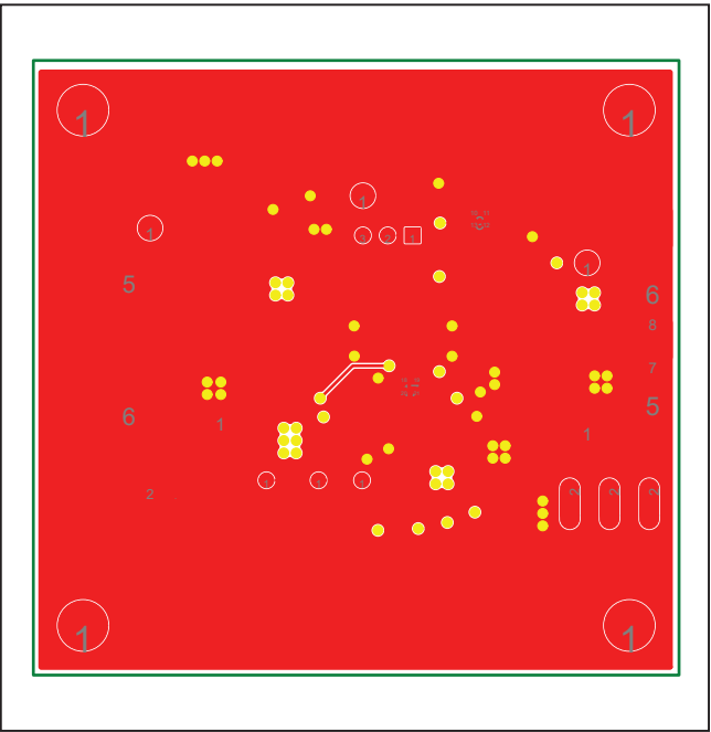
MAX16972A EV Kit PCB Layout (TQFN)—Solder Side
