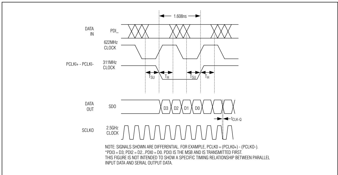
Figure 1. Timing Diagram
