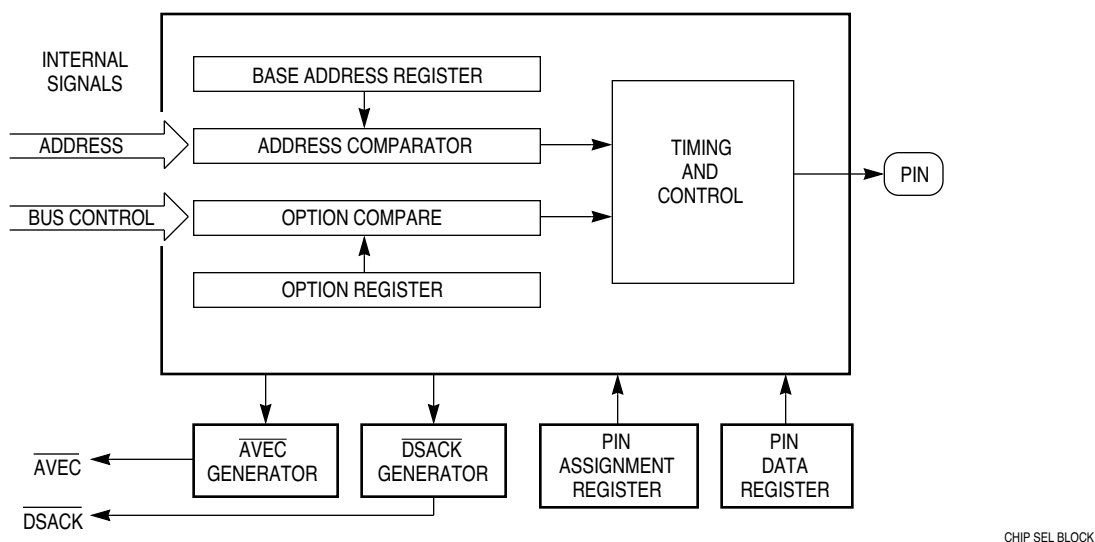
Figure 9 Chip-Select Circuit Block Diagram
