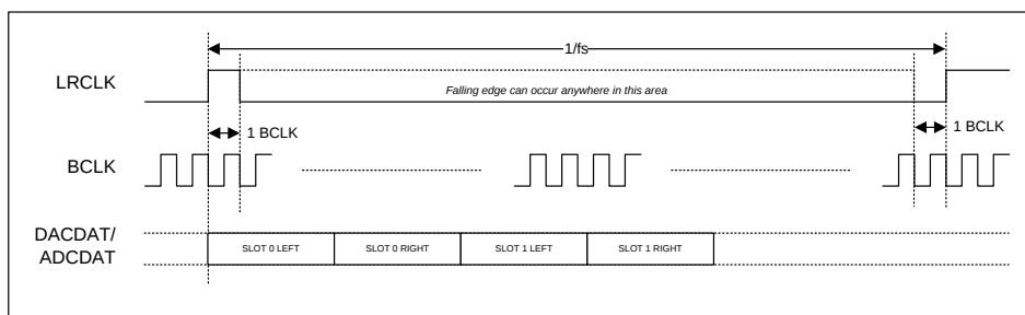
Figure 54 TDM in DSP Mode B
