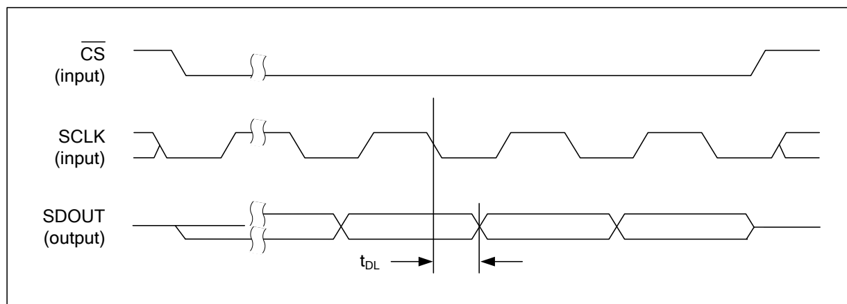
Figure 10 Control Interface Timing - 4-wire (SPI) Control Mode (Read Cycle)
