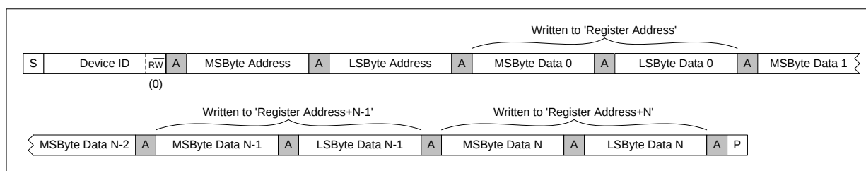
Figure 67 Multiple Register Write to Specified Address using Auto-increment
