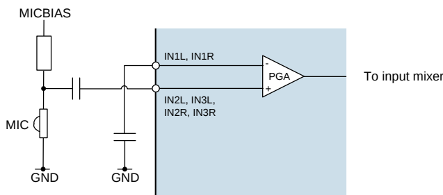
Figure 15 Microphone Input IN2 or IN3
