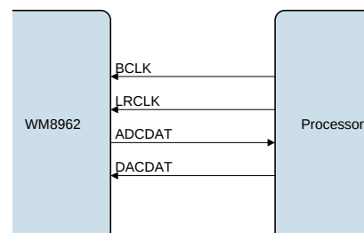
Figure 39 Slave Mode
