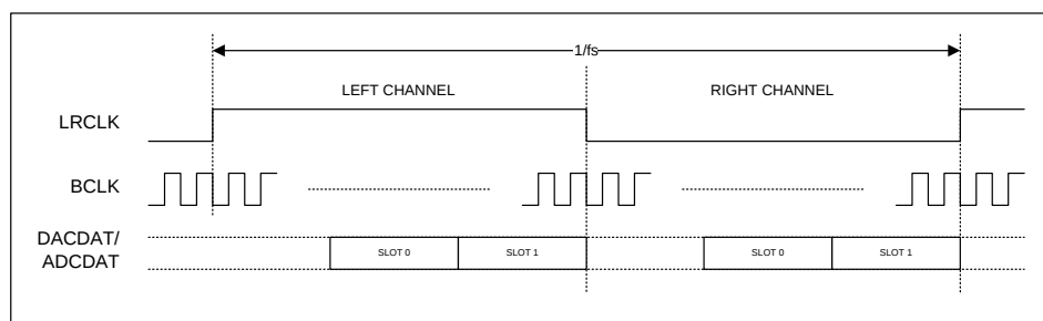
Figure 50 TDM in Right-Justified Mode
