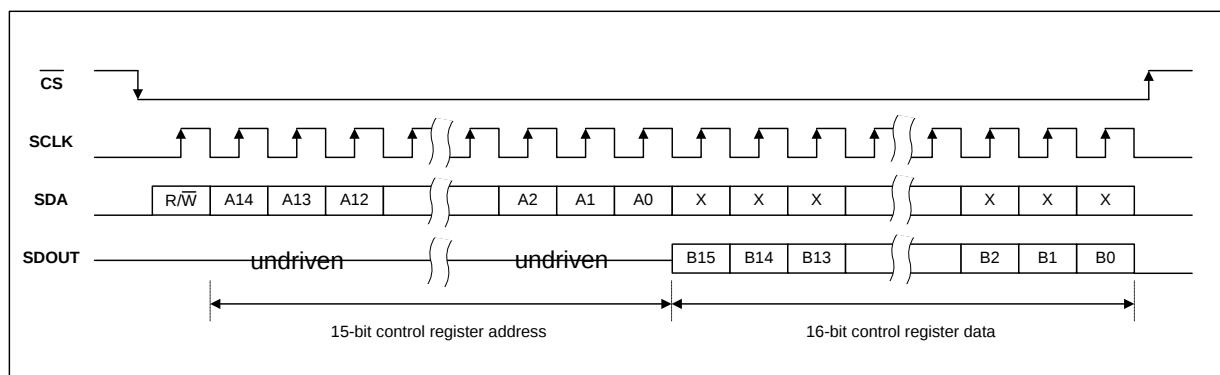
Figure 72 4-Wire Readback (Wired-'OR')
