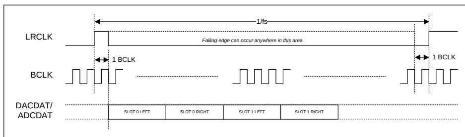
Figure 53 TDM in DSP Mode A
