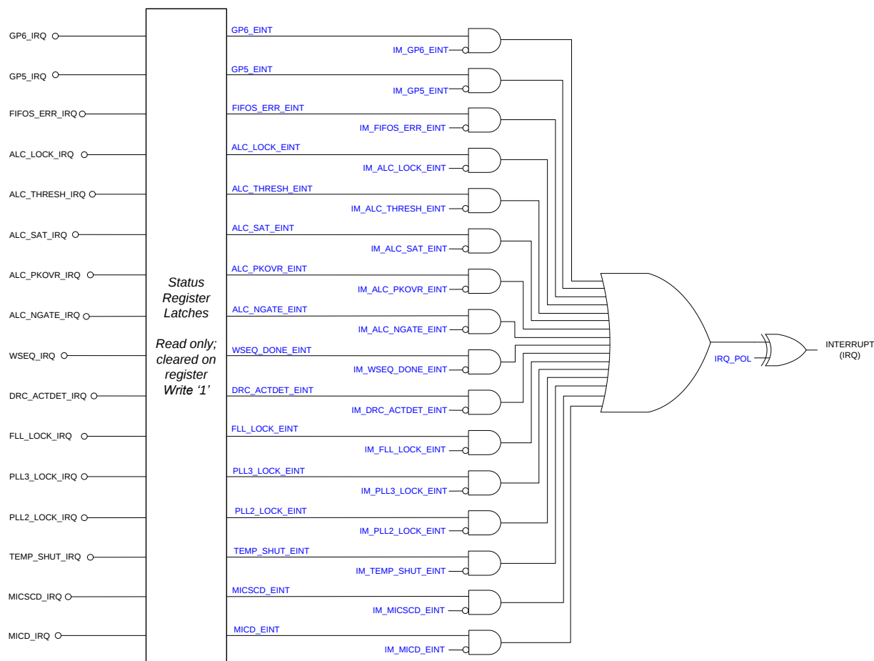
Figure 62 Interrupt Controller
