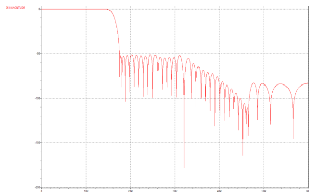
Figure 80 DAC Playback Filter Response for 32k Sample Rate
