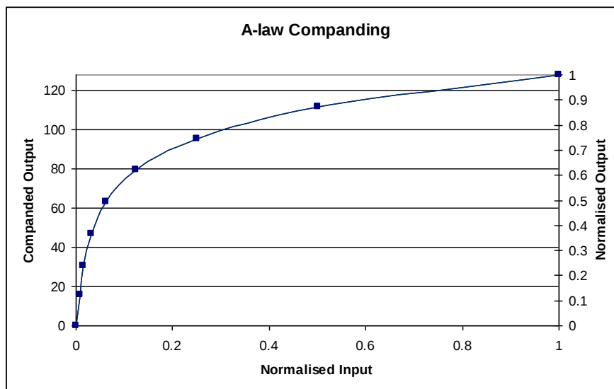
Figure 56 A-Law Companding
