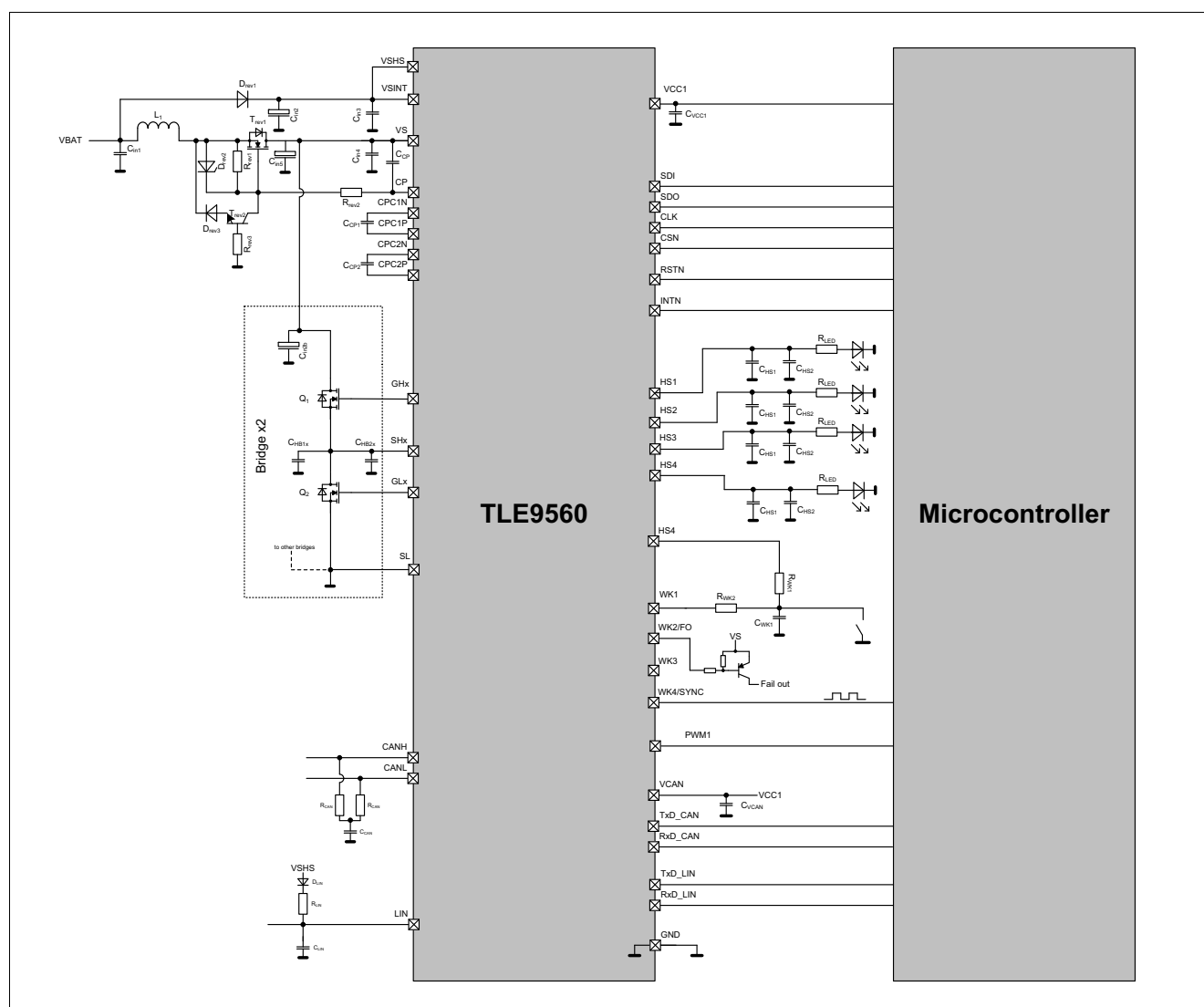
Figure 95 TLE9560-3QX Application Diagram
