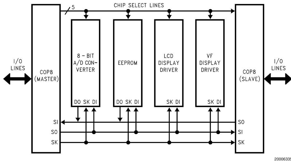
FIGURE 34. MICROWIRE/PLUS Application
