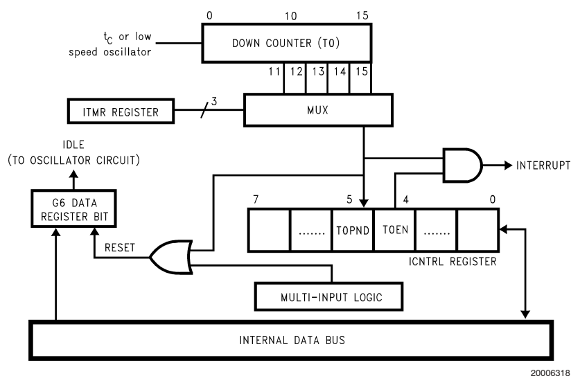
FIGURE 14. Functional Block Diagram for Idle Timer T0
