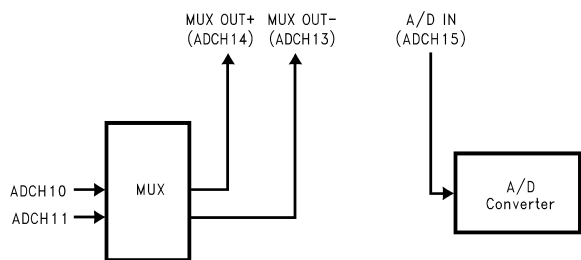
FIGURE 27. A/D with Differential Mux Output Feature Enabled
