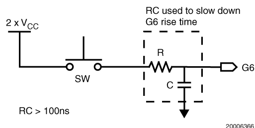
FIGURE 13. Circuit Diagram for Implementing the 2 \times V_{CC}
