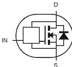
Device Symbol
