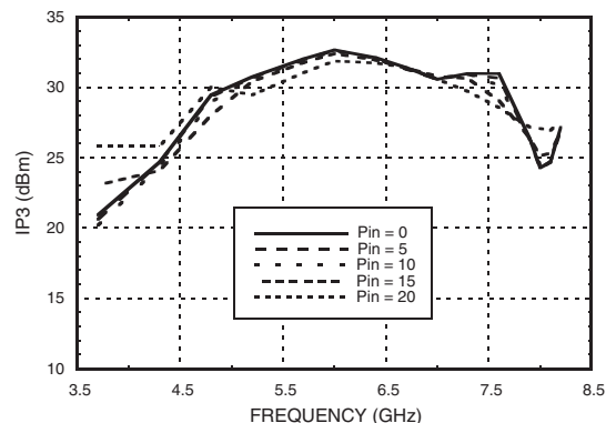
Input IP3 vs. Power Input V fctl = V bwctl
