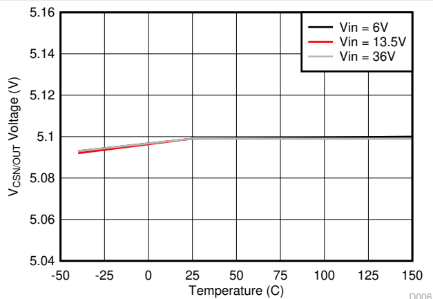
Figure 8-7. V_{CSN/OUT} Voltage vs Junction Temperature
