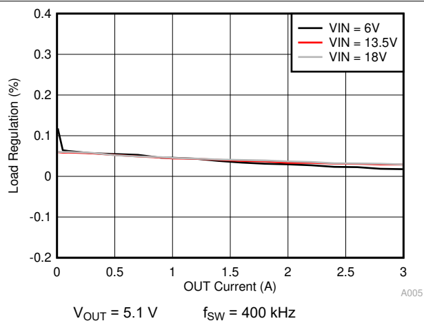
Figure 11-6. Load Regulation
