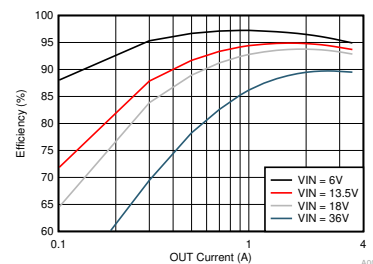
Buck Efficiency vs Output Current f_{\text{sw}} = 400 \text{ kHz}
