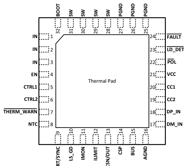
Figure 7-4. TPS25831QCWRHBRQ1 Package 32-Pin (VQFN) Top View (2)
