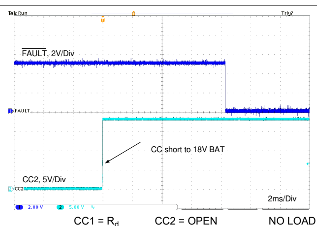
Figure 11-33. CC Short to BAT
