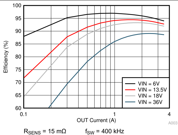
Figure 11-4. Efficiency With Sense Resistor
