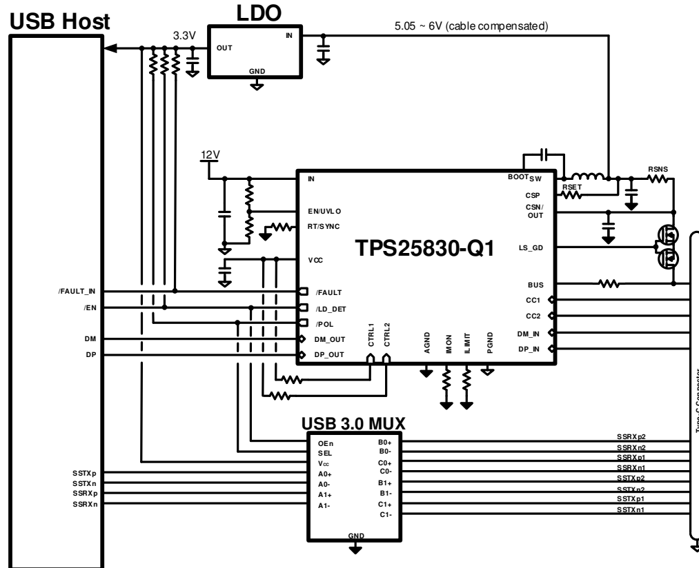
Figure 10-27. Example Implementation
