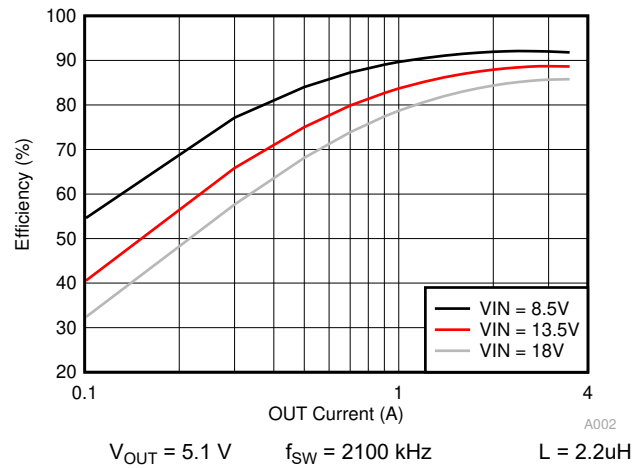
Figure 11-3. Buck Only Efficiency
