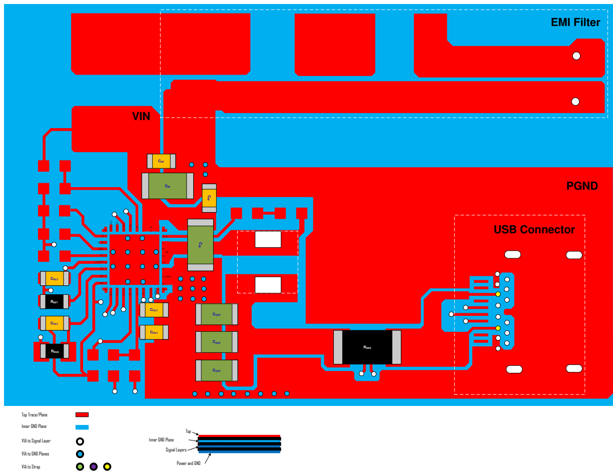
Figure 13-1. Layout
