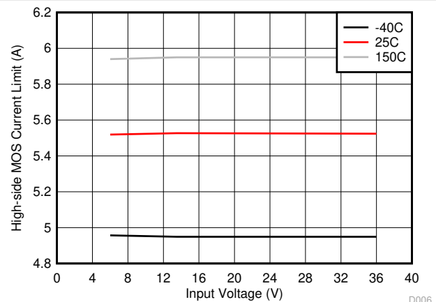
Figure 8-8. High-side Current Limit vs Input Voltage
