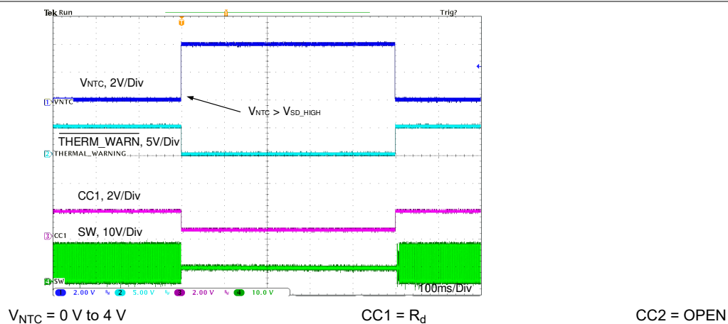
Figure 11-38. Thermal Sensing With NTC Behavior 2
