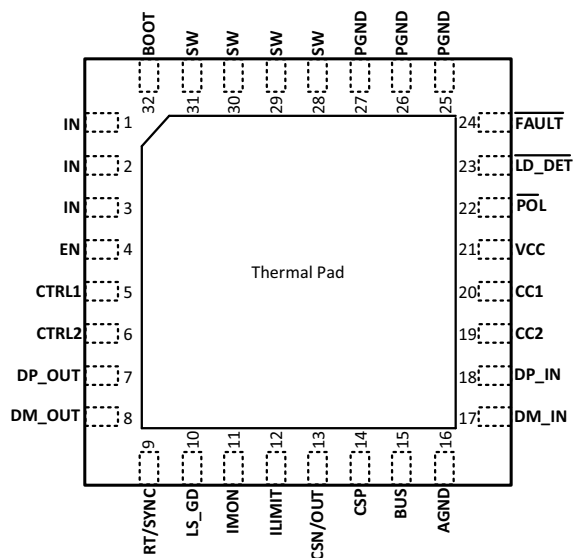
Figure 7-3. TPS25830QCWRHBRQ1 Package 32-Pin (VQFN) Top View (2)
