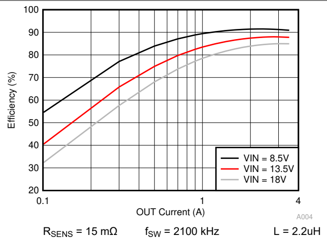
Figure 11-5. Efficiency With Sense Resistor
