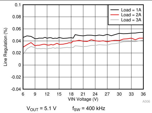
Figure 11-7. Line Regulation
