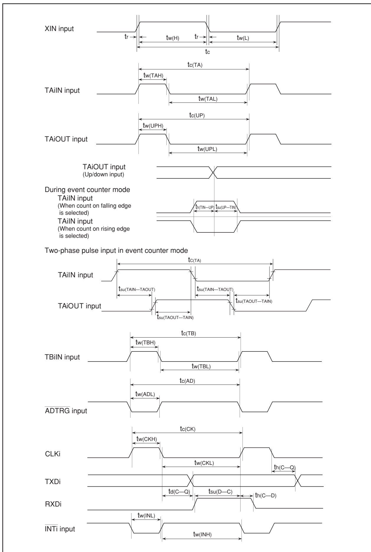
Figure 5.4 Timing Diagram (1)
