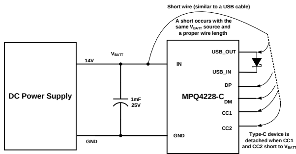
Figure 8: Short-to-Battery Set-Up
