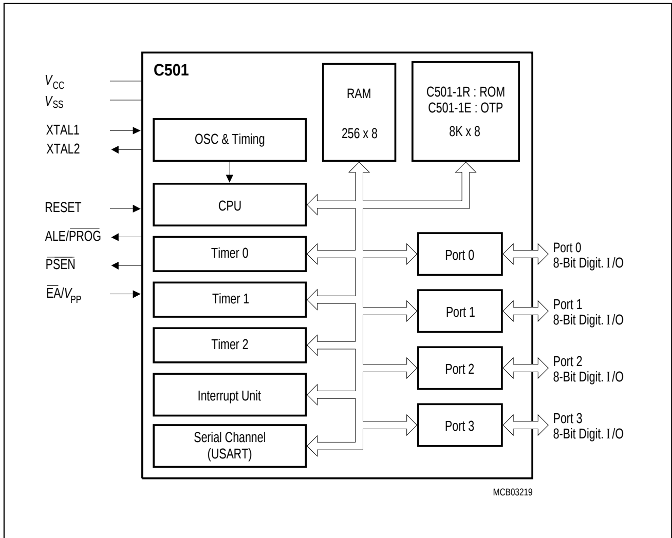
Figure 6 Block Diagram of the C501
