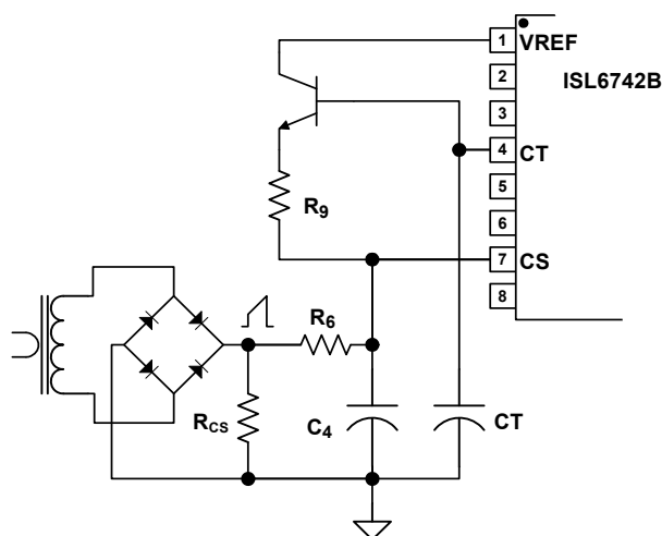
FIGURE 17. ADDING SLOPE COMPENSATION
