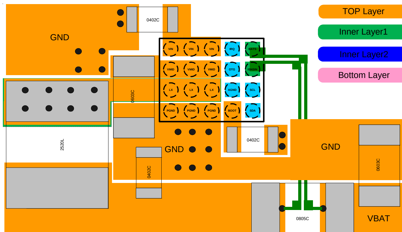
Figure 3. PCB Layout Guide
