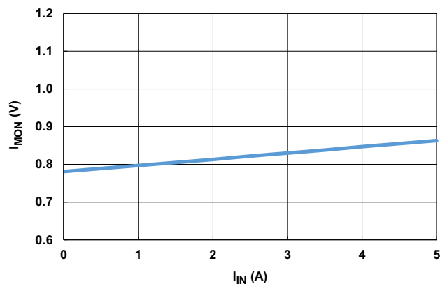
Figure 19. Dual-Phase Input Current IIN (DC) vs IMON1 Pin Voltage, RS_IN = 4mΩ, RIM_IN = 20kΩ
