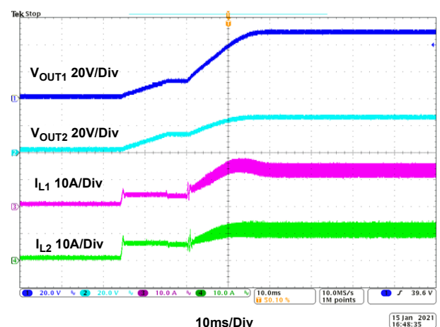
Figure 36. Dual Output Waveforms, Start-Up Waveform, V_{IN} = 12V , V_{OUT1} = 48V , V_{OUT2} = 24V , I_{OUT1} = 3A , I_{OUT2} = 5A , CCM
