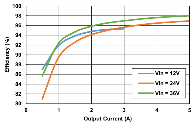
Figure 21. CCM Mode Efficiency
