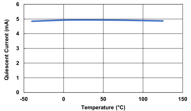
Figure 9. Quiescent Current vs Temperature
