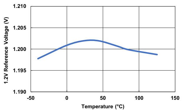
Figure 17. 1.2V Reference Voltage vs Temperature
