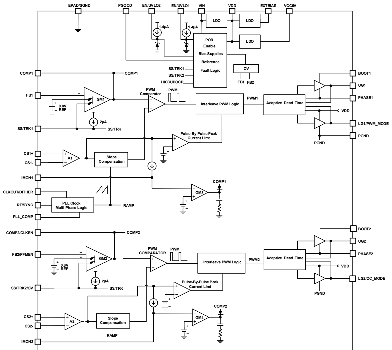
Figure 7. Block Diagram
