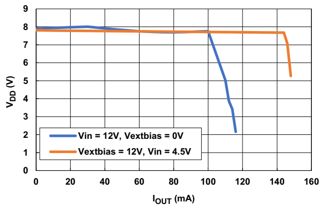
Figure 10. V_{DD} Load Regulation at 12V Input
