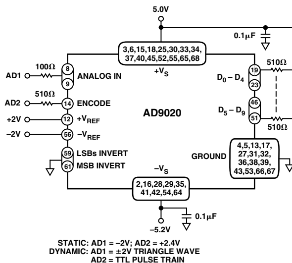
Figure 1. Burn-In Circuit
