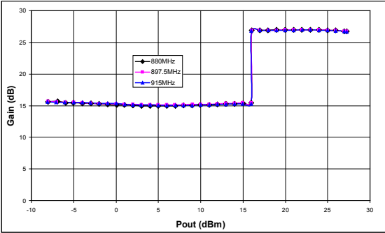
Figure 8: Gain vs Output Power
