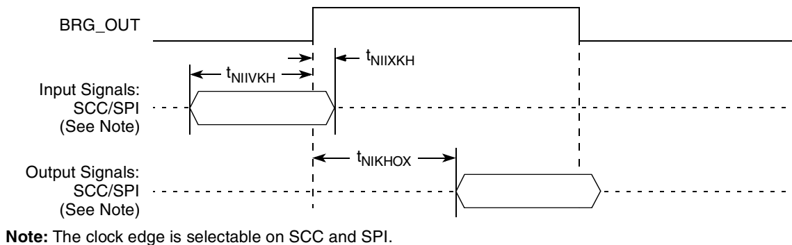
Figure 28. SCC/SPI AC Timing Internal Clock Diagram
