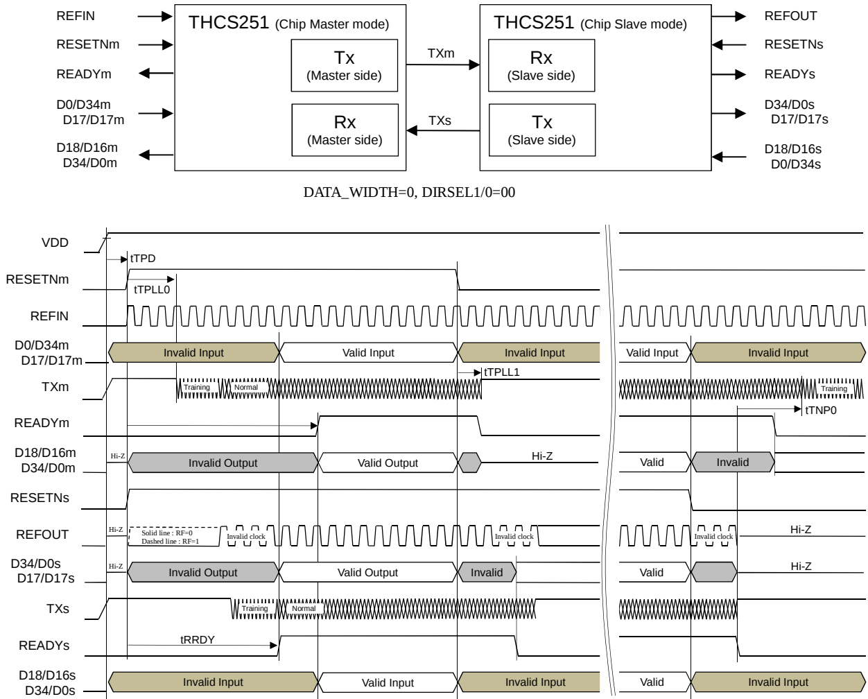
Figure 6 GPIO/CML Bi-directional mode Power on & Reset timing diagram
