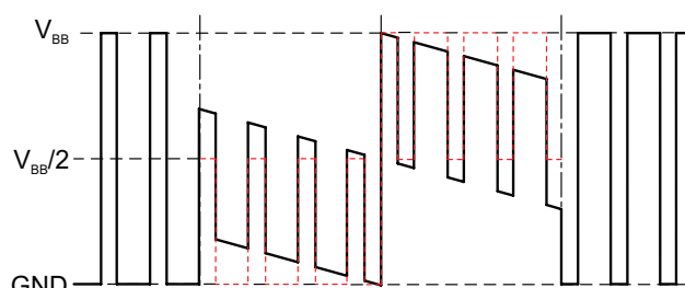
Figure 18d: Auto Mixed Recirculation, bemf Falling
