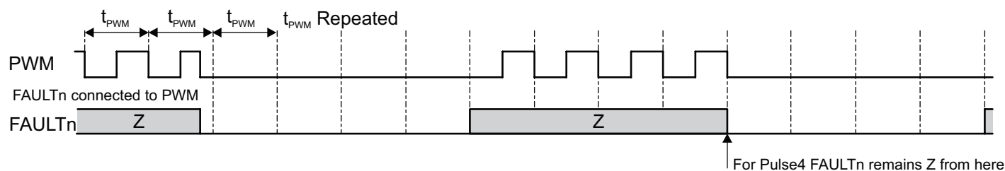
Figure 22: Indirect Mode PWM – Overtemperature Fault Output Timing (Pulse4R) (IPI = 0)
