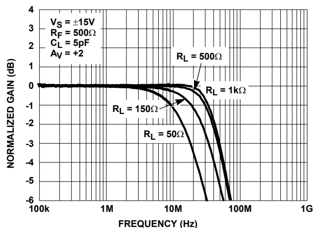
FIGURE 10. GAIN vs FREQUENCY FOR VARIOUS R_{LOAD} ( A_V = +2 )
