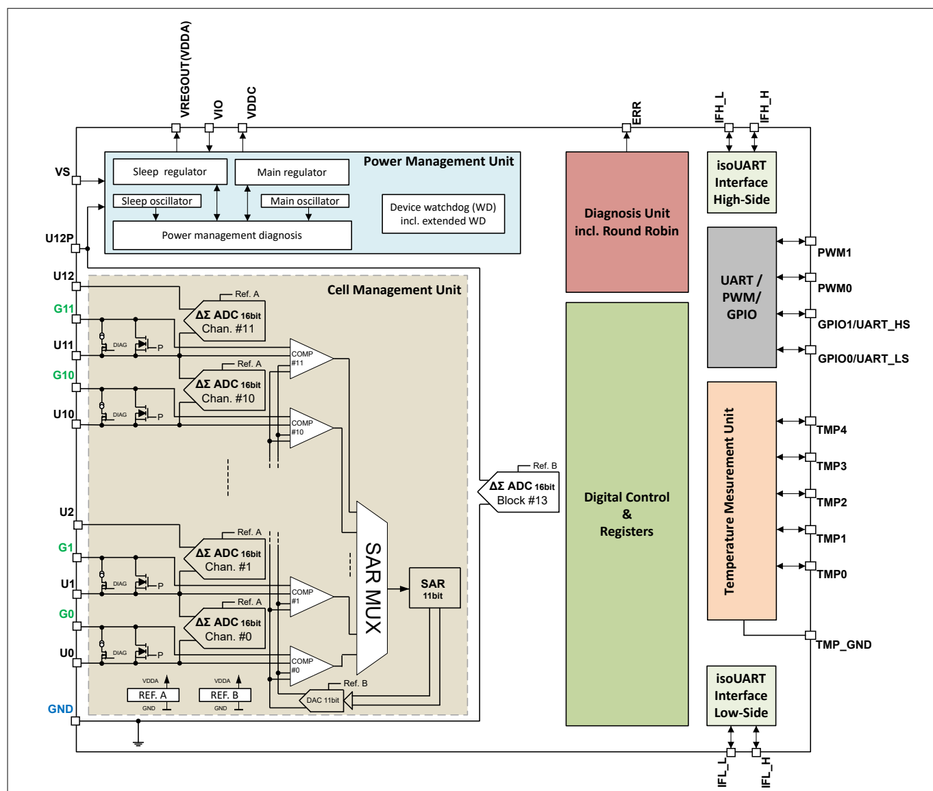
Figure 1 Block diagram
