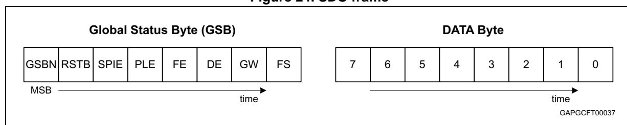
Figure 24. SDO frame
