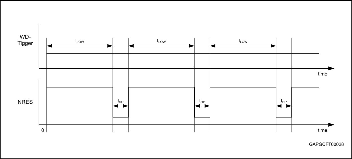
Figure 16. Watchdog missing
