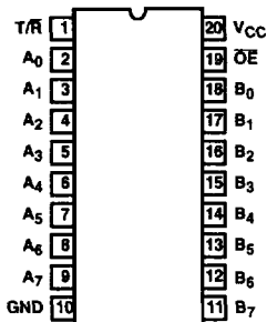
CD74LPT245 (QSOP, SOIC) TOP VIEW
