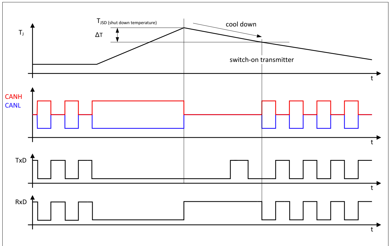
Figure 8 Overtemperature protection
