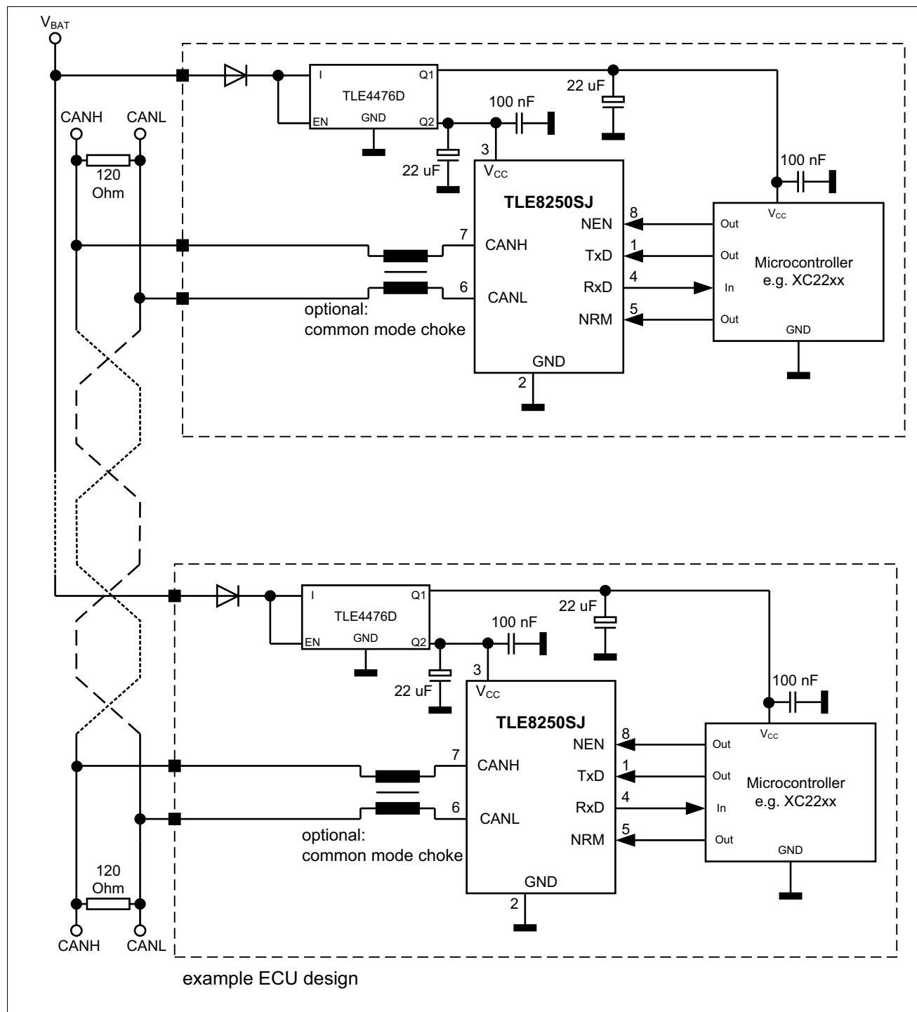
Figure 12 Application circuit
